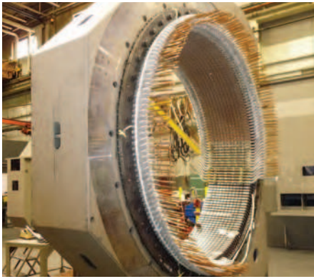
Generator stator winding in process
