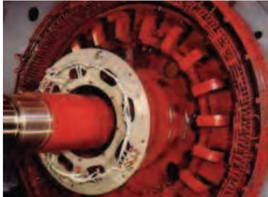
Rotor and stator in final assembly.
